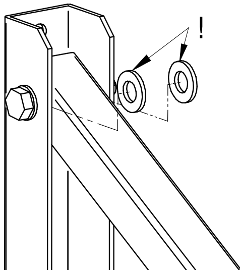
GA8575 Horizontal mounting consoles a
