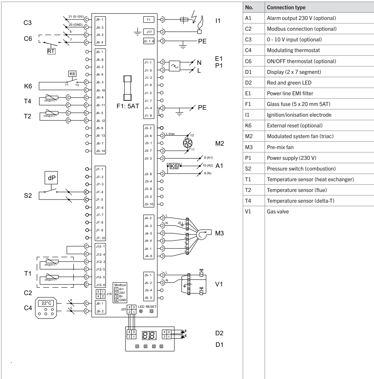
Figure 23 - Electrical wiring diagram AC
