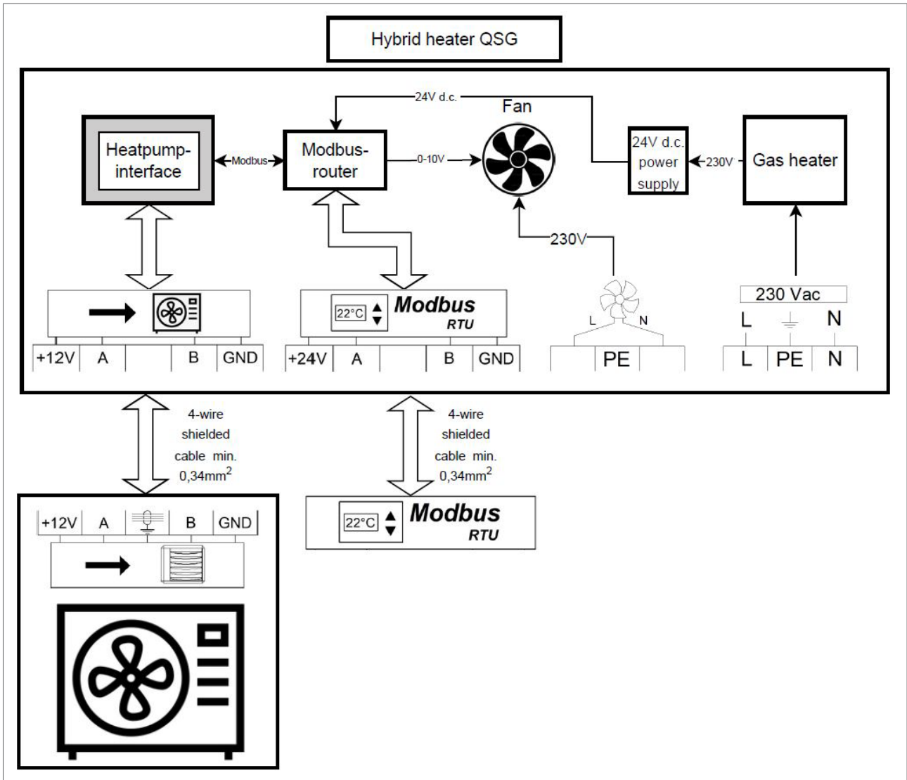
Figure 24 - Electrical diagram of the QSG
